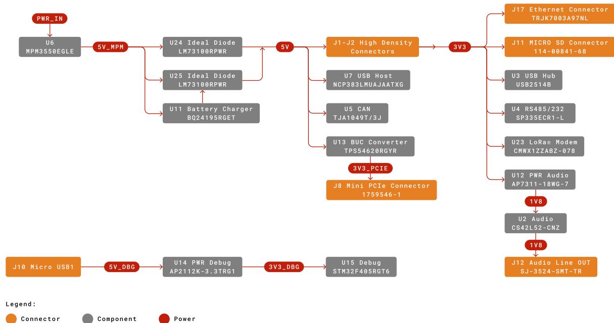
Power tree
